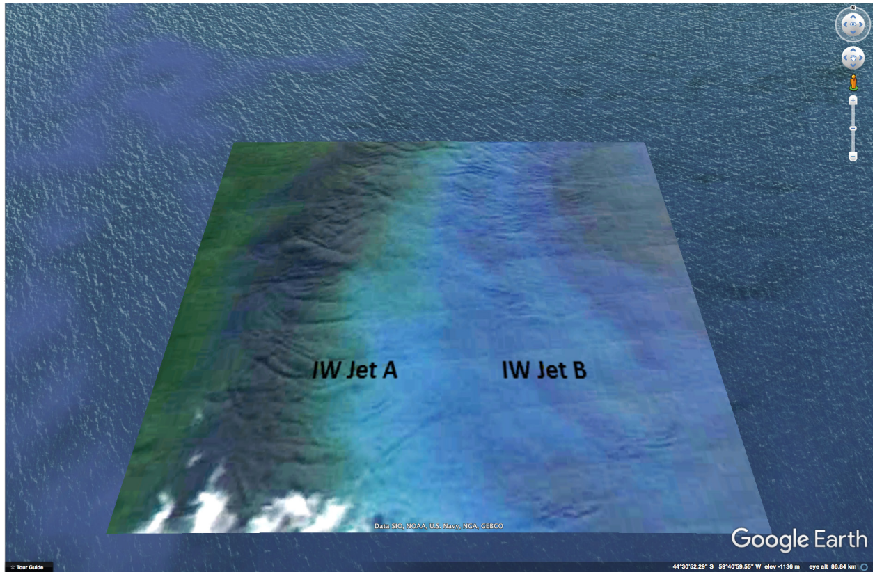
FIGURE S4. An RGB composite from a MODIS-Aqua acquisition dated January 6, 2014, at 17:45 UTC.
