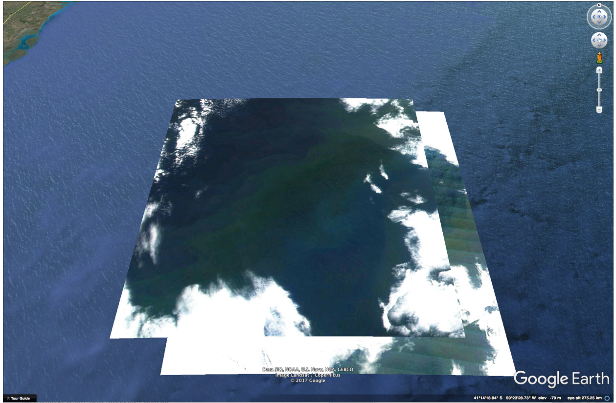
FIGURE S3. A synergy between two RGB composites dated January 31, 2016, acquired at 14:00 UTC (MODIS-Terra) and 17:20 UTC (Suomi-Viirs).
