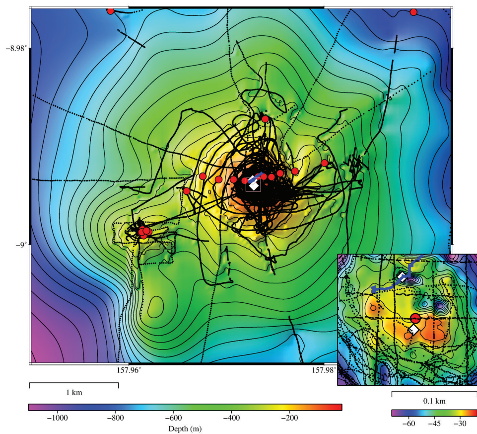
FIGURE S1. Bathymetric map of Kavachi and the summit crater (inset, lower right) showing locations of single-beam echosounder returns used to create the plot (black dots). See the Methods section for a detailed description of how the bathymetric data was processed.
