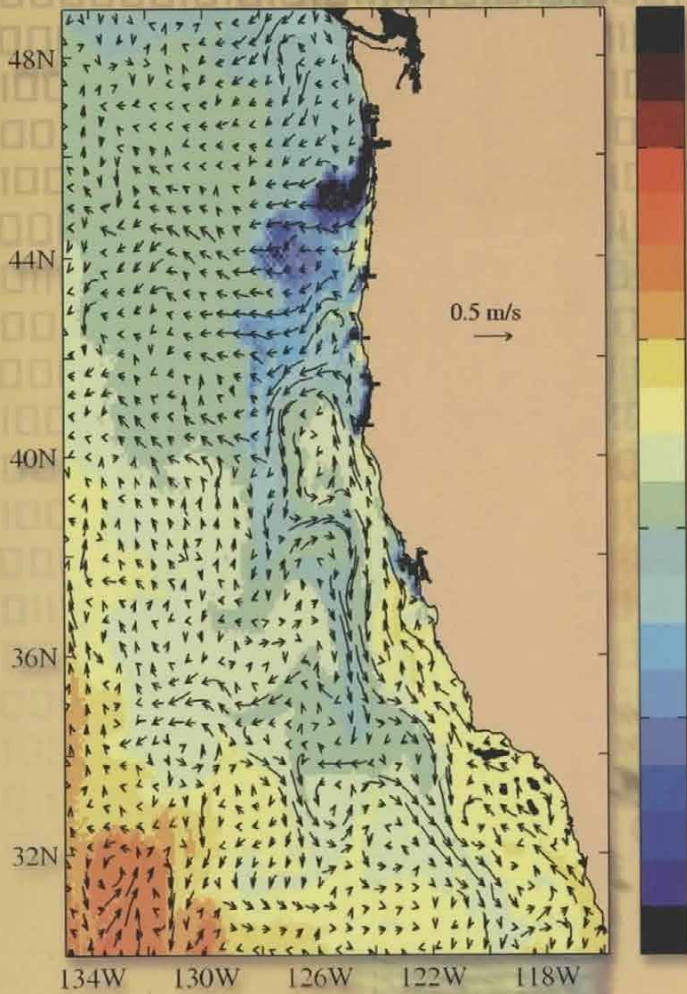
SALINITY AND 10m CURRENTS 13 - July - 1996
