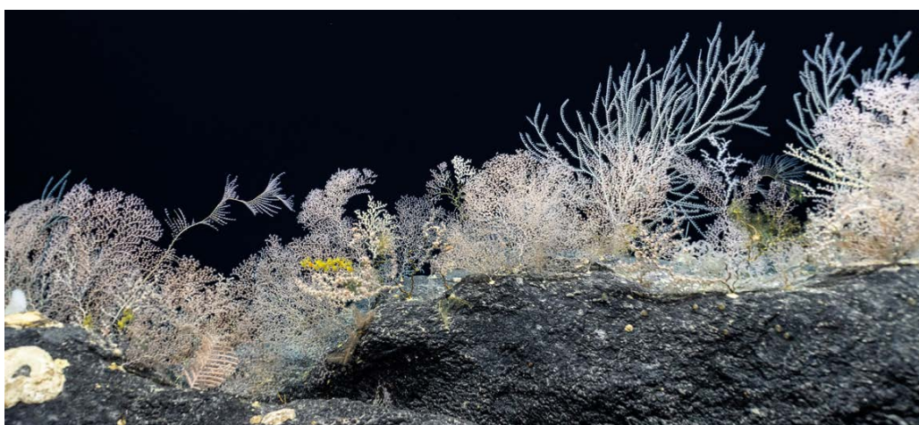
FIGURE 4. An outcrop observed at 1,895 m depth on an unnamed seamount during dive H1930 harbors a high density of golden and bamboo corals, as well as Poliopogon sp. glass sponges.
