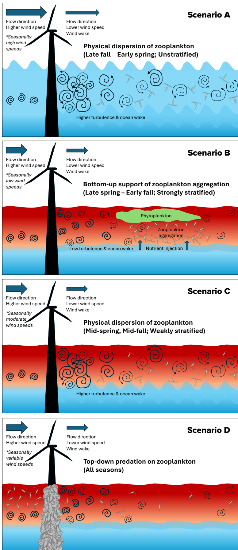
FIGURE 1. Four potential scenarios of offshore wind turbulence and wake effects on zooplankton in Nantucket Shoals waters.
