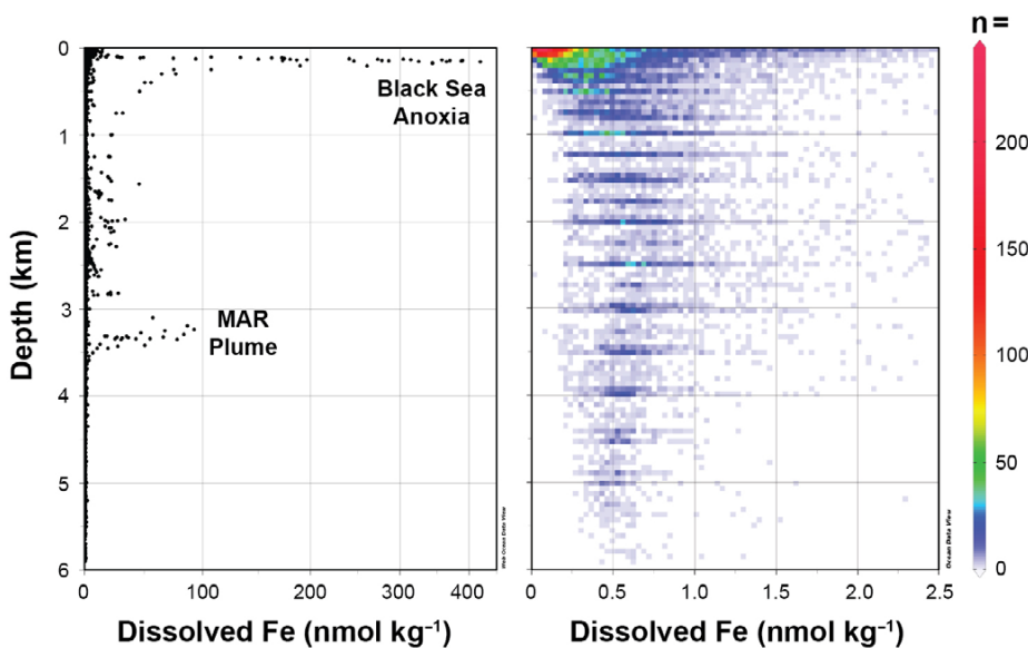
FIGURE 1. Distribution of all dissolved Fe concentration data included in the GEOTRACES Data Product 2021v2 (GEOTRACES Intermediate Data Product Group, 2023). The data show ranges from 0.01 to 420 \text{nmol kg}^{-1} , with the most elevated values associated with Fe sources (anoxic Black Sea waters and/or Mid-Atlantic Ridge [MAR] hydrothermal plumes), and most data falling between 0 and 1 \text{nmol kg}^{-1} . Note nonlinear x axis on left-hand panel.
