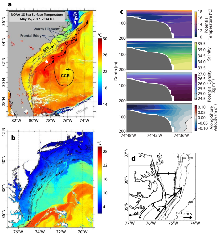
FIGURE 2. (a) Sea surface temperature (SST) image offshore of the South Atlantic Bight (SAB) with Gulf Stream meander crests (C) and troughs (T) labeled, and a white star marking the position of the Charleston Bump. MAB = Mid-Atlantic Bight. CCR = Cold Core Rings. Image from Rutgers University (b) SST image of the Gulf Stream and Slope Sea offshore of the Mid-Atlantic Bight shelf. Image from Rutgers University (c) Average shelfbreak temperature, salinity, density, and along-shelf velocity during PEACH measured along the cross-shelf section in Figure 3. After Todd (2020), Figure 7 (d) Mean flow convergence near Cape Hatteras. From Savidge and Bane (2001)
