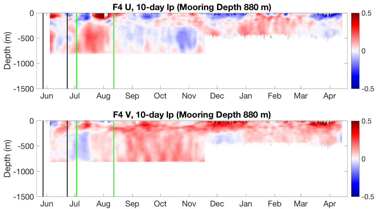
FIGURES S3. Zonal (top) and meridional (bottom) currents ( \text{m s}^{-1} , shaded) 10-day low-pass filtered as measured at F4 at the northern edge of Velasco Reef from June 2016 through April 2017. As in Figure 7.
