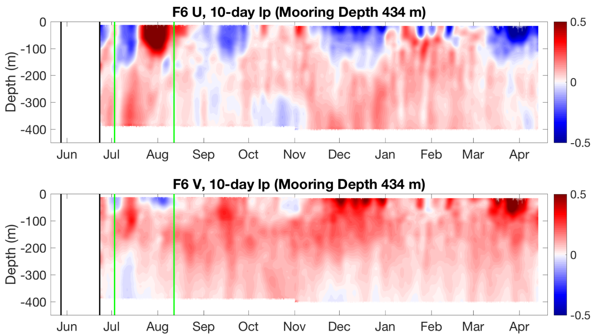
FIGURES S4. Zonal (top) and meridional (bottom) currents ( \text{m s}^{-1} , shaded) 10-day low-pass filtered as measured at F6 at the northern edge of Velasco Reef from June 2016 through April 2017. As in Figure 7.
