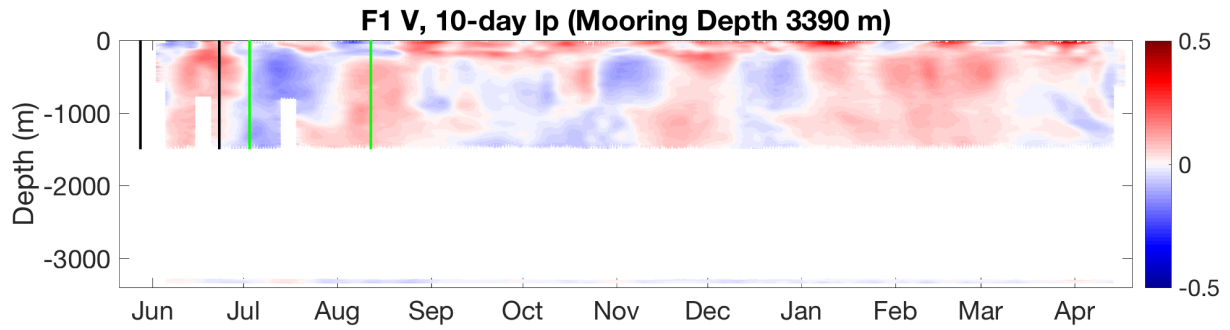
FIGURES S1. Zonal (top) and meridional (bottom) currents ( \text{m s}^{-1} , shaded) 10-day low-pass filtered as measured at F1 at the northern edge of Velasco Reef from June 2016 through April 2017. As in Figure 7.
