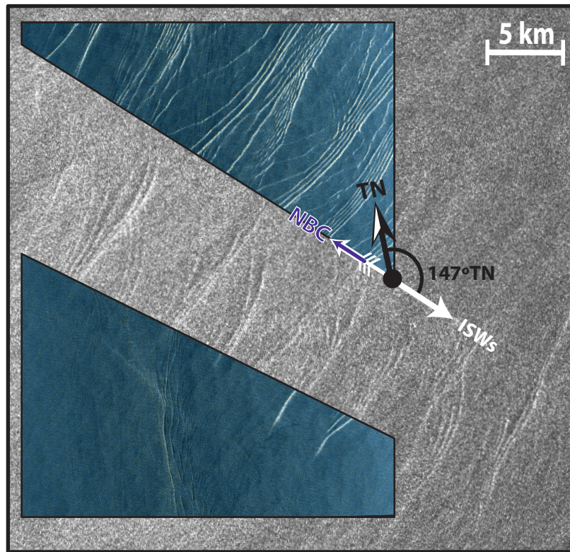
FIGURE S1. Subset from a RADARSAT image dated March 25, 1999, acquired at 9:11 UTC. Selected sections from Figure 1b are overlaid to highlight the consistency of the two-dimensional ISW structure.
