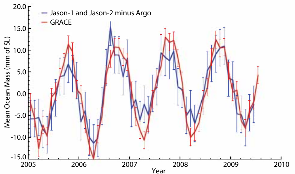
Figure 4. Ocean mass measured from the time-variable gravity satellite mission GRACE (Gravity Recovery And Climate Experiment, red) and inferred from steric-corrected Jason-1 and Jason-2 altimetry (blue). The steric correction is calculated from Argo data with all potentially biased float data removed. To allow for adequate global coverage by Argo, the inferred estimate of ocean mass is computed only for the years from 2005 on. The most recently released Jason-1 and Jason-2 data (GDR-C) were used here, and the GRACE data were corrected for GIA using the model recommended in Chambers et al. (in press). The excellent agreement suggests that the three observing systems, Jason, GRACE, and Argo, are accurate enough to capture total sea level variation and its causes on these time scales. The seasonal cycle is dominated by the yearly exchange of water between ocean and land related to the hydrologic cycle. The trend between 2005 and 2010 is 1.3 \pm 0.6 \text{ mm yr}^{-1} .
