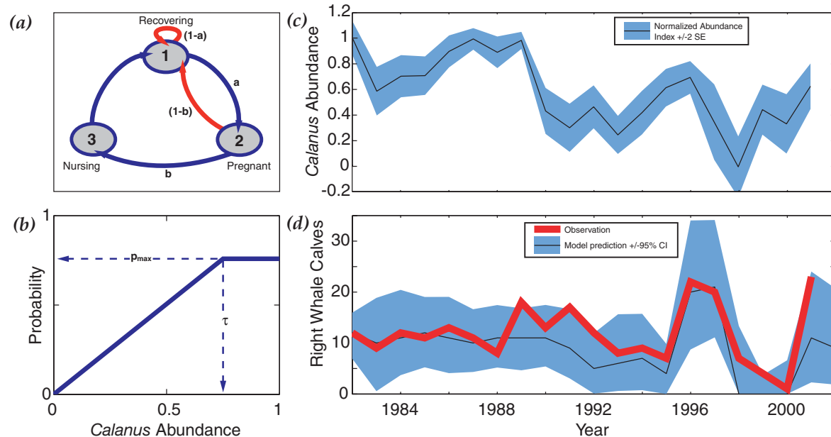
Figure 3. Right whale reproduction model. a) Diagram of reproductive cycle, with transitional probabilities between states indicated. A whale in any of the three states, pregnant, nursing, or recovering, will move to the next state with a probability determined by Calanus finmarchicus abundance in that year. If reproduction is unsuccessful, then the animal will move to the recovery state. b) The transitional probabilities are simple functions of Calanus finmarchicus abundance as described by two parameters, \tau , the saturating food level, and p_{\max} , the maximum transitional probability. Parameter values were selected using a genetic algorithm to yield the best agreement between predicted and observed calving rates. c) The Calanus finmarchicus Abundance Index as determined from Continuous Plankton Recorder surveys in the Western Gulf of Maine. d) Number of right whale calves observed (red) and predicted by the model (blue). The blue region encompasses the 95% confidence interval surrounding the model predictions. Contact authors for further details.
