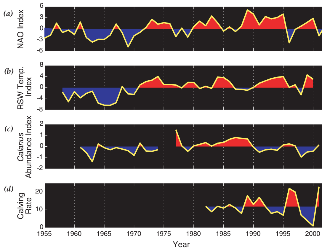
Figure 2. Time series from the North Atlantic. a) Annual values of the winter NAO Index. b) Annual values of the Regional Slope Water Temperature Index. c) Annual values of the Calanus finmarchicus Abundance Index. d) Annual values of right whale calving rate. The winter NAO Index is the mean atmospheric pressure difference between the North Atlantic's subtropical high-pressure system, measured in Lisbon, Portugal, and the subpolar low pressure system, measured in Stykkisholmer, Iceland (Hurrell, 1995). The Regional Slope Water Temperature Index is an indicator of the modal state of the CSWS, with positive (negative) values corresponding to maximum (minimum) modal state conditions (MERCINA, 2001). It is the dominant mode derived from a principal components analysis of eight slope water temperature anomaly time series from the GOM/WSS region. The Calanus finmarchicus Abundance Index is the mean abundance anomaly for this species calculated each year as the mean difference between log-transformed observed abundances and log-transformed expected abundances (MERCINA, 2001). Abundance data were derived from Continuous Plankton Recorder surveys conducted in the GOM/WSS region since 1961. Right whale calving rate is the number of individually identified females accompanied by calves observed during a year beginning in December of the preceding calendar year. Data through 2001 were provided by S.D. Kraus, New England Aquarium. Contact authors for further details
