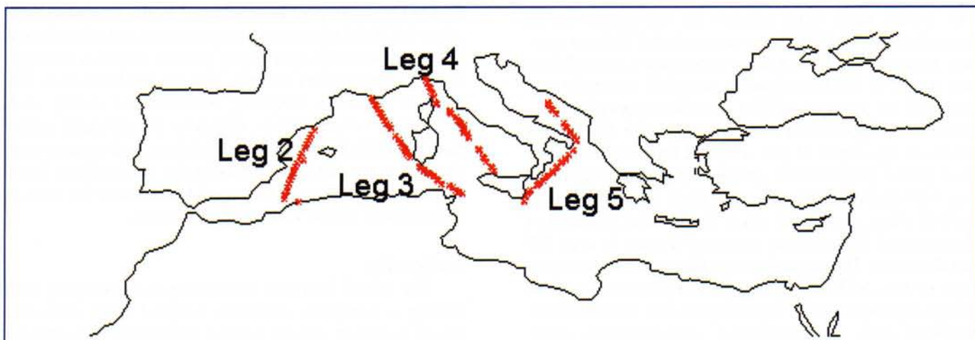
Figure 5. Mediterranean Forecast System Pilot Project XBT drops during October 1999. The XBT samples were made along sections which, from west to east, are referred to as Leg 2, Leg 3, Leg 4, and Leg 5.
