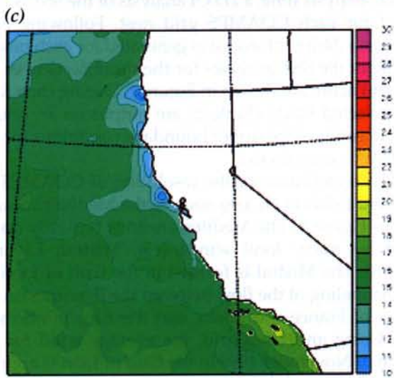
Figure 1. COAMPS sea surface temperature analyses using 2-dimensional optimum interpolation analysis at 0000 UTC 1 July 1999 for a) 81 km grid, b) 27 km nest, and c) 9 km nest.
