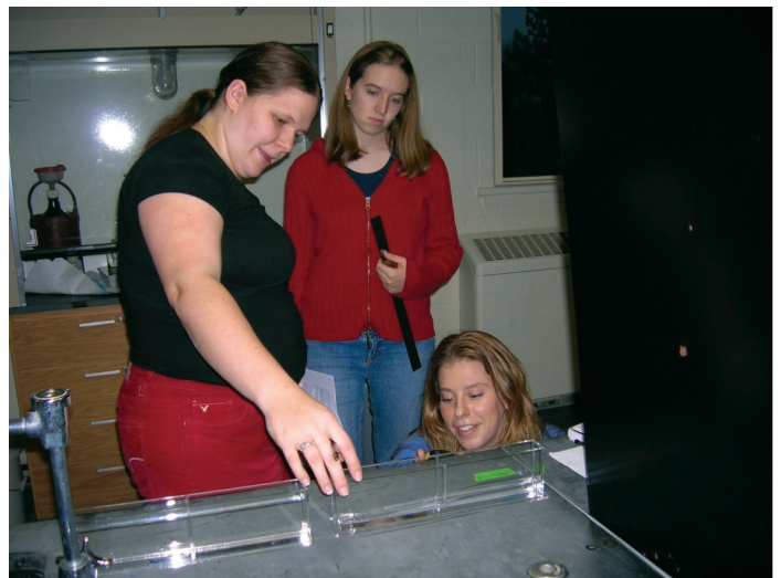
Figure 5.1. Wave speed and wave depth. Students measure the number of “sloshes” in a tank filled with water to a depth of 1.5 cm.
