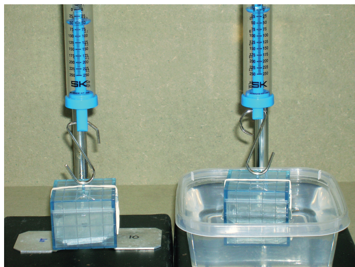
Figure 3.1. Apparatus for Activity 3.1 in air (left, with two weights lying on the table) and in water (right).
